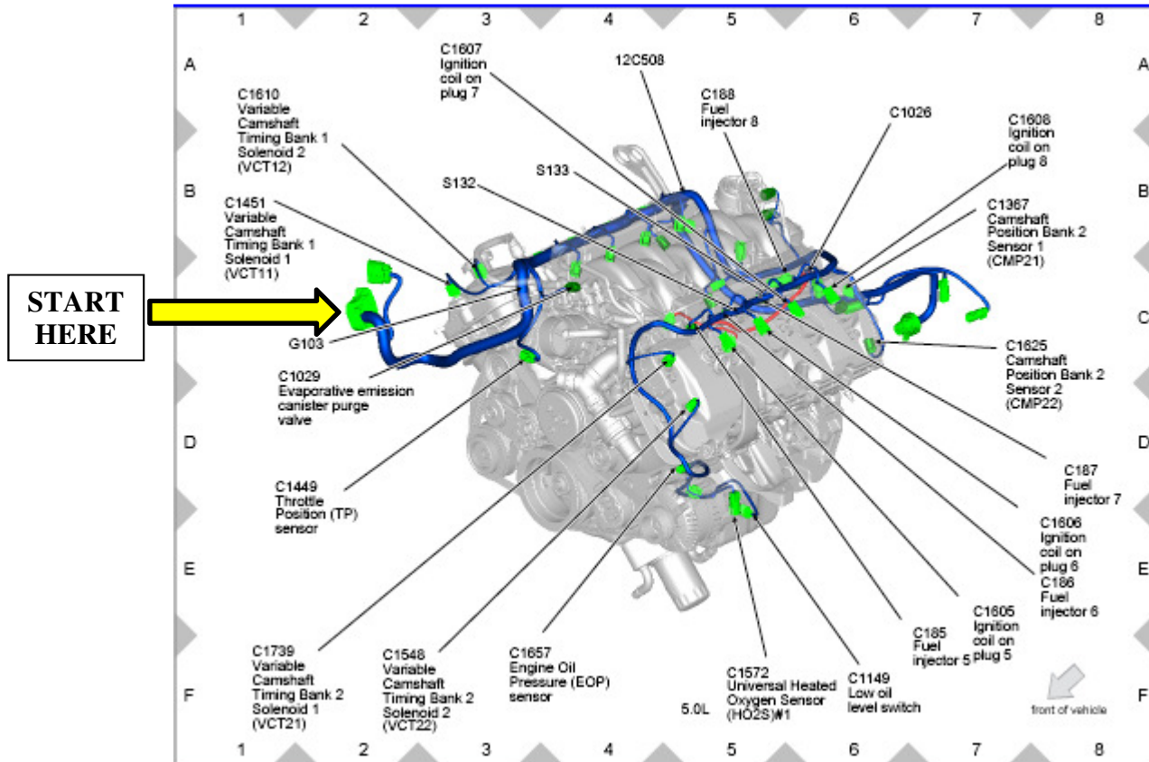
Figure 3 – Rear View of Engine.
