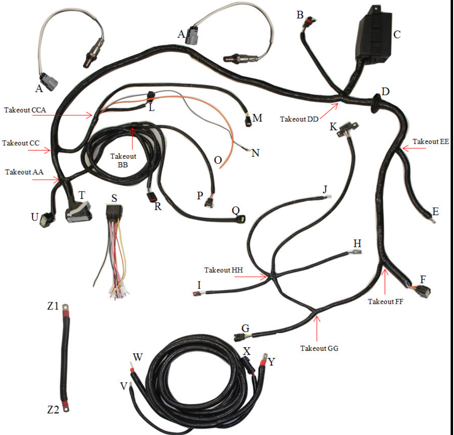
Figure 1 - Controls Pack Wiring Harness Components
