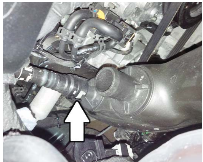
11. Remove the PCV quick connect fitting from the stock clean air tube.
